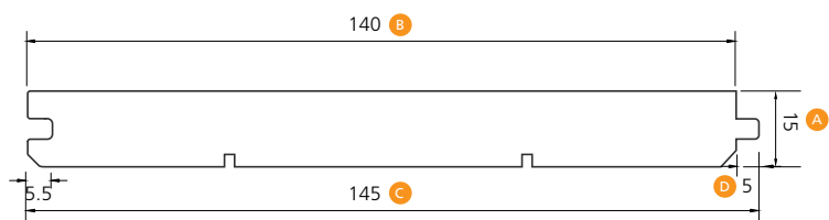
Section – Typical Tongue and Groove Profile
